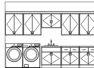
Cabs. above W & D & Sink Option
