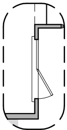
Center Hinge ILO Sliding Glass Door
