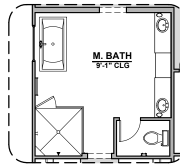
Tub w/ Glass Shower
